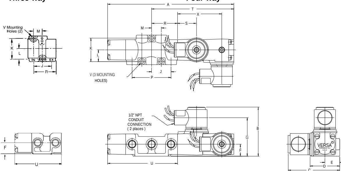
Three-way
