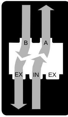
Inlet open to cylinder port A, cylinder port B open to exhaust.
