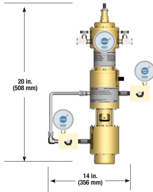
Figure 5 - Overall dimensions of Becker Model VRP-600-SB-CH Pilot Control System (Direct-Acting)
